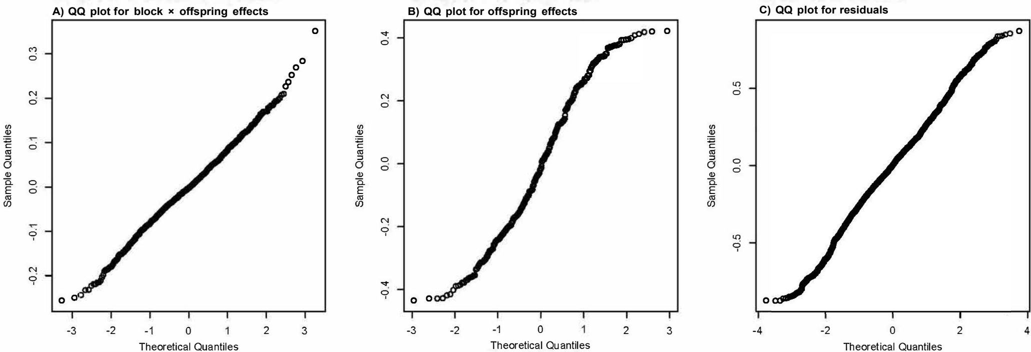
Figure S5. Normal QQ (i.e., sample versus theoretical quantiles) plots used to check normality of random effects (i.e., block \times offspring interaction, offspring) and residuals of the mixed linear model fit to 2016 shoot length blighted (SLB) data described by Kostick et al. 1
